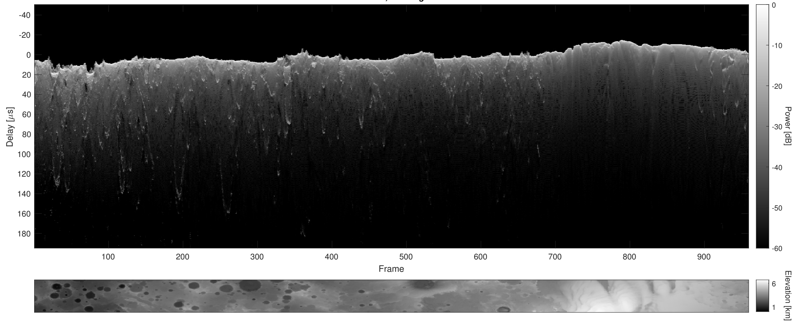
Orbit 6754, Cluttergram
