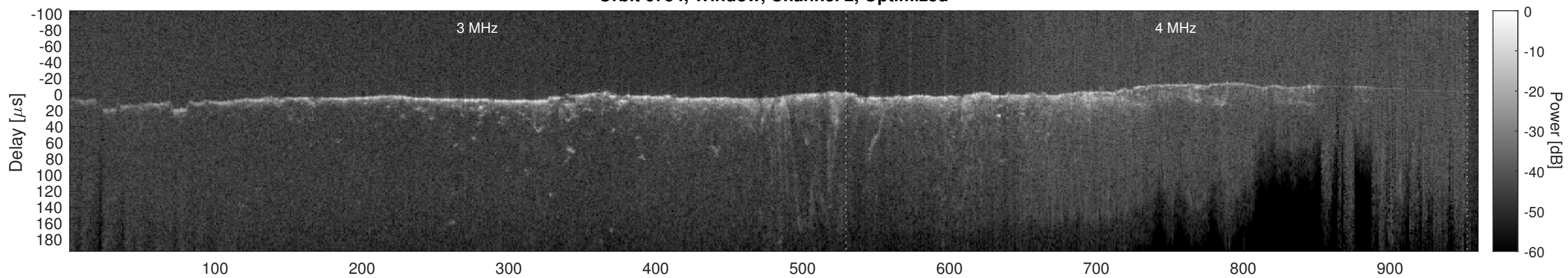
Orbit 6754, Cluttergram
