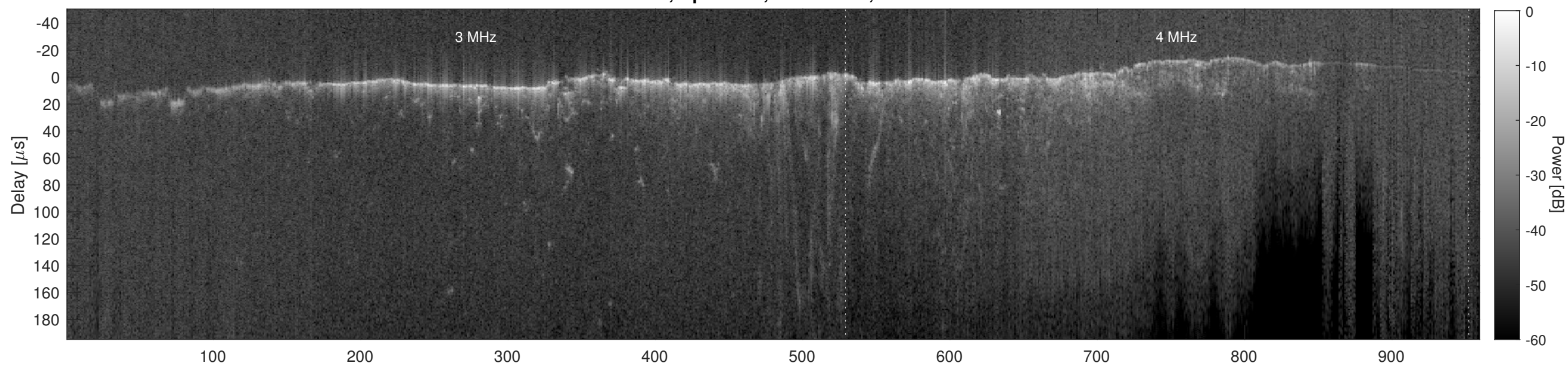
Orbit 6754, Cluttergram
