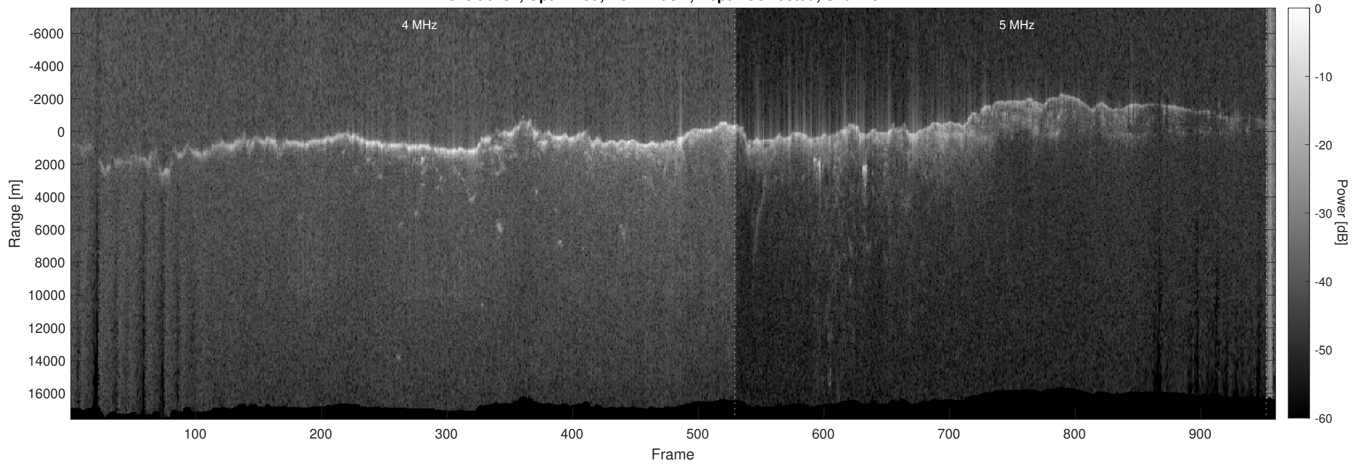
Orbit 6754, Optimized, No Window, Depth-Corrected, Channel 2
