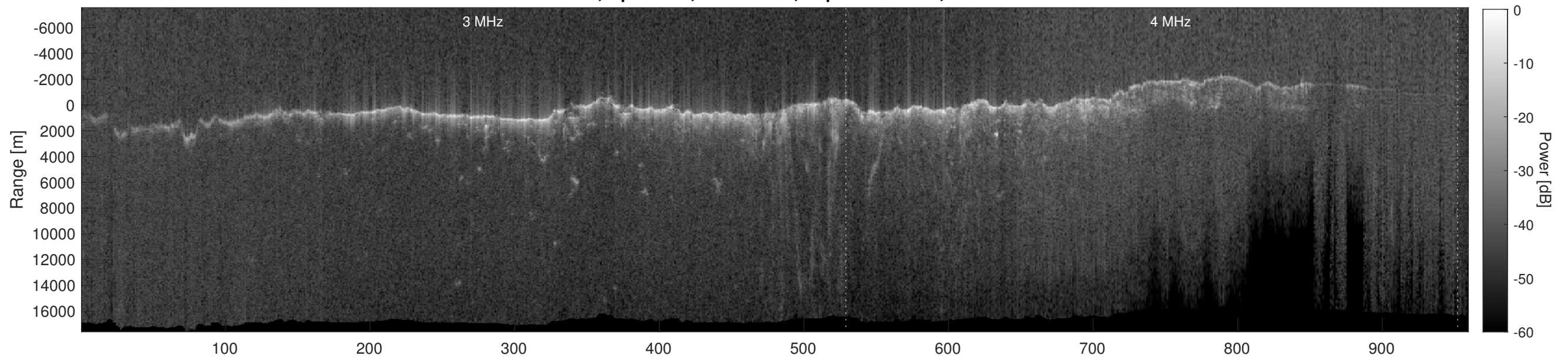
Orbit 6754, Depth-Corrected Cluttergram
