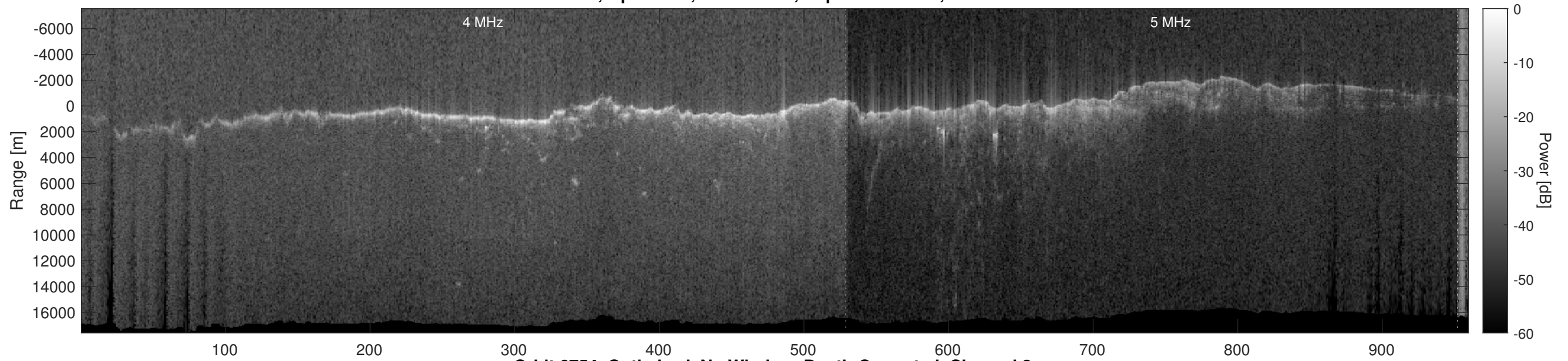
Orbit 6754, Optimized, No Window, Depth-Corrected, Channel 2
