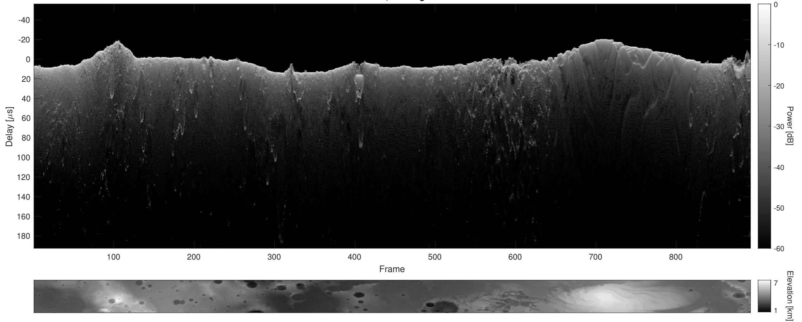
Orbit 6755, Cluttergram
