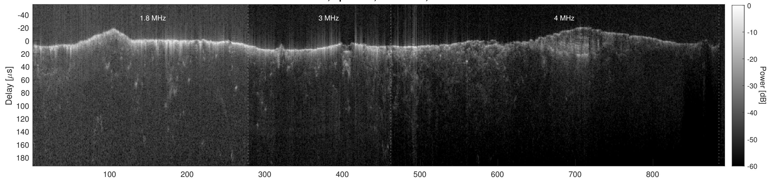
Orbit 6755, Cluttergram
