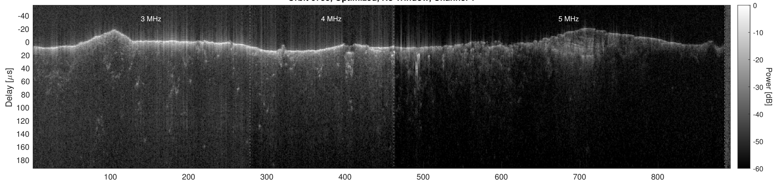
Orbit 6755, Optimized, No Window, Channel 2
