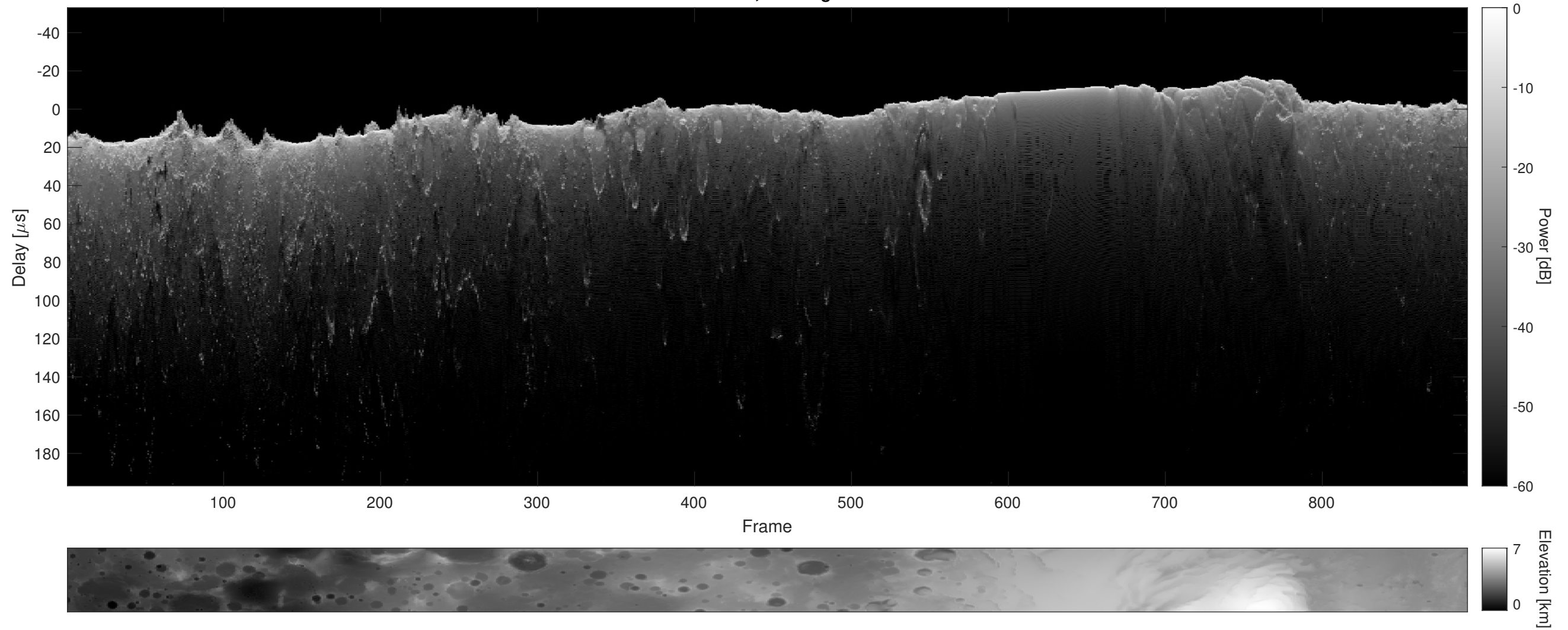
Orbit 6756, Cluttergram
