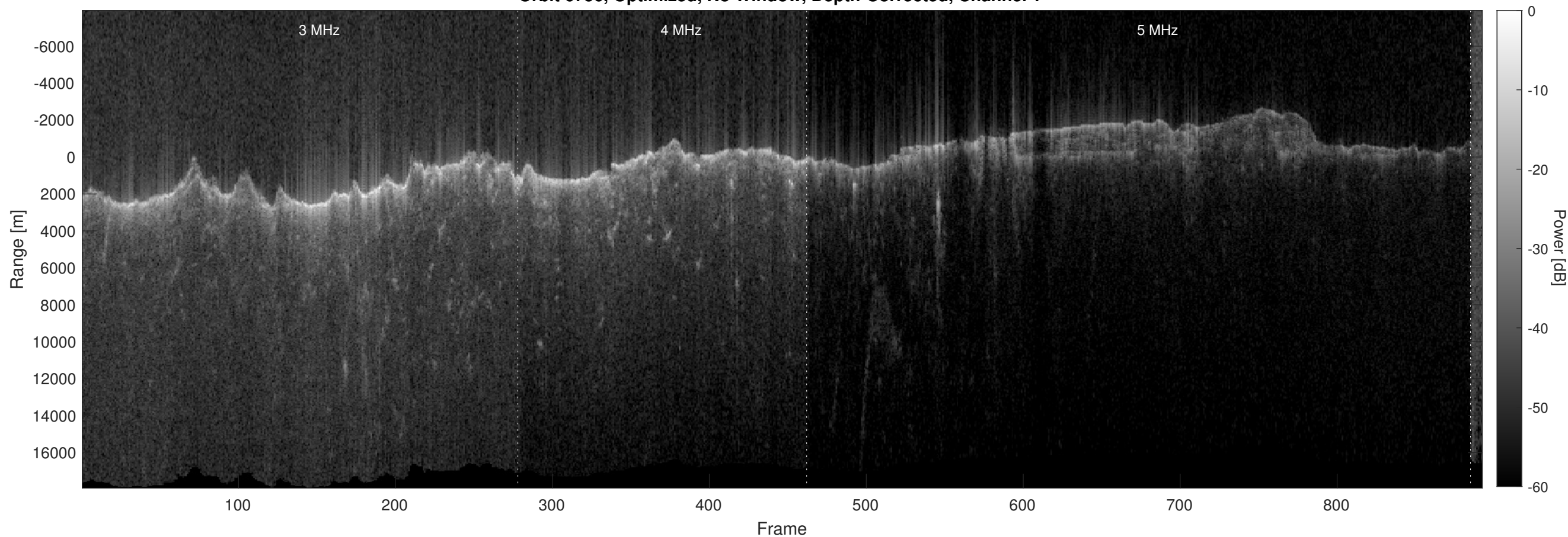
Orbit 6756, Optimized, No Window, Depth-Corrected, Channel 2
