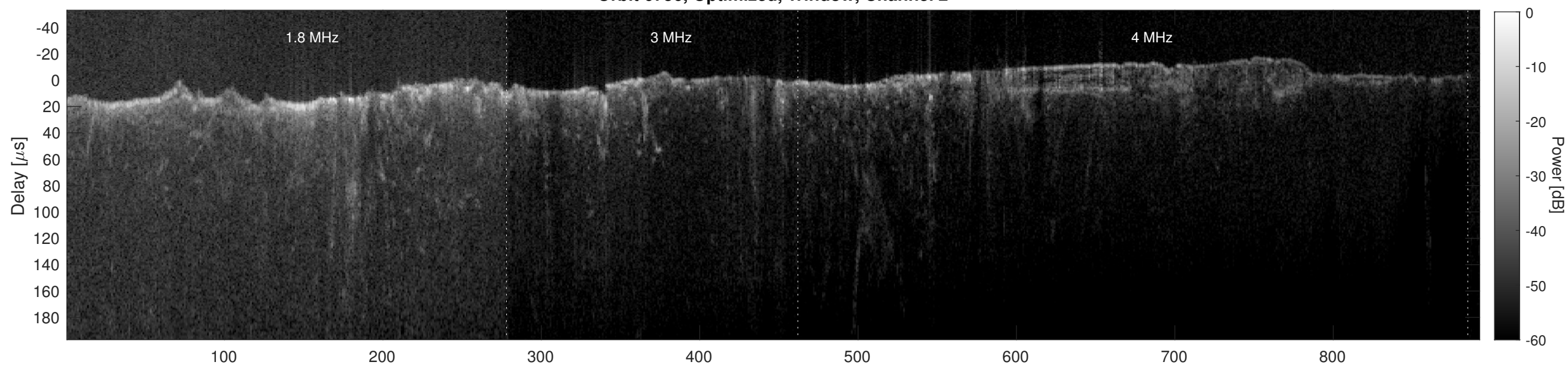
Orbit 6756, Cluttergram
