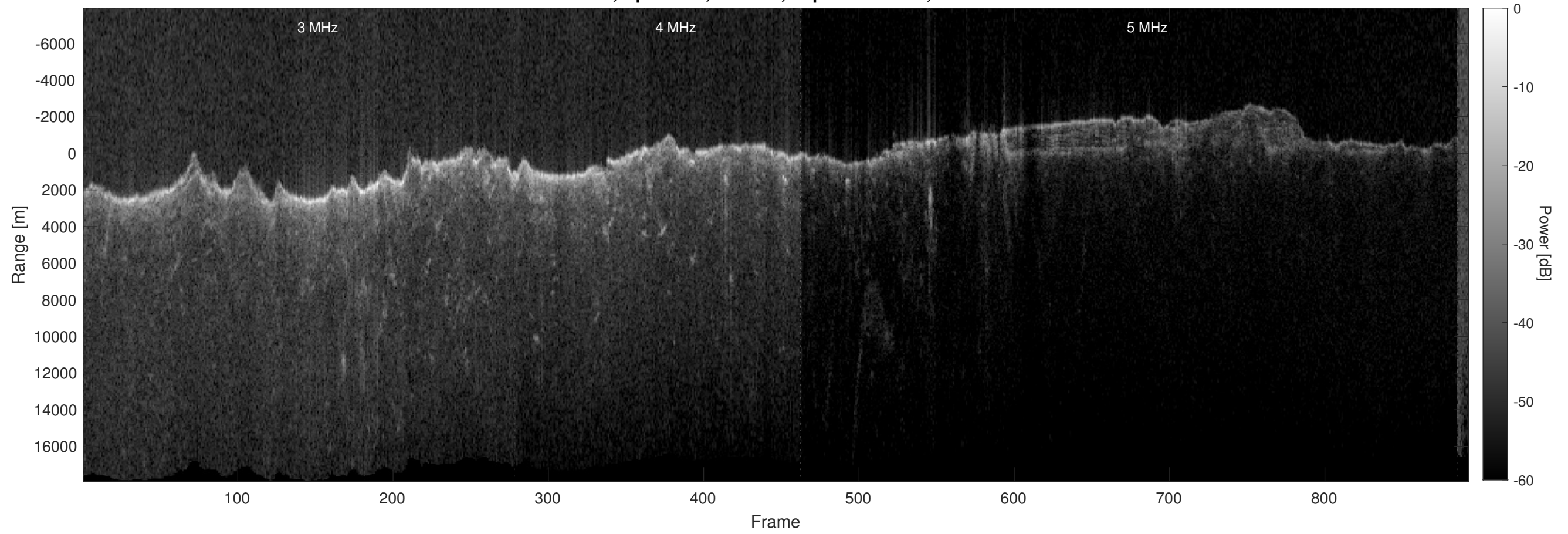
Orbit 6756, Optimized, Window, Depth-Corrected, Channel 2
