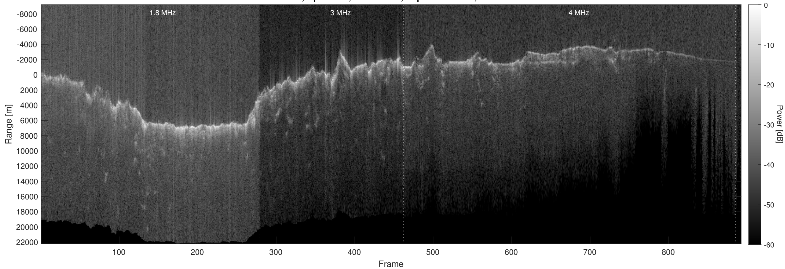
Orbit 6757, Optimized, No Window, Depth-Corrected, Channel 2
