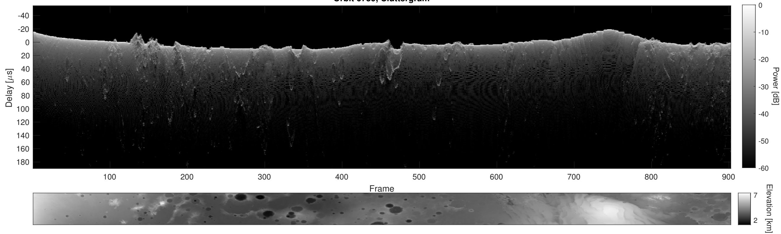
Orbit 6759, Cluttergram
