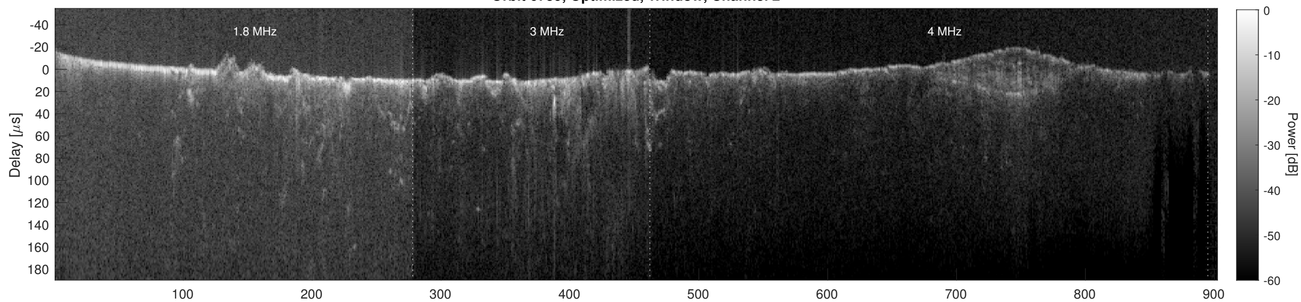
Orbit 6759, Cluttergram
