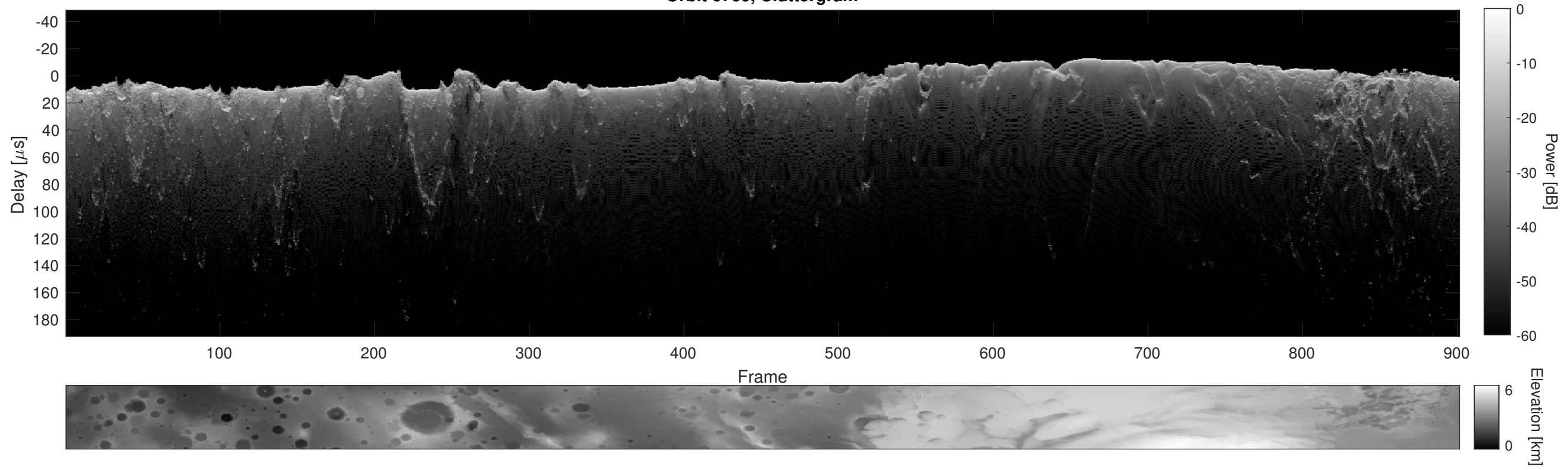
Orbit 6760, Cluttergram
