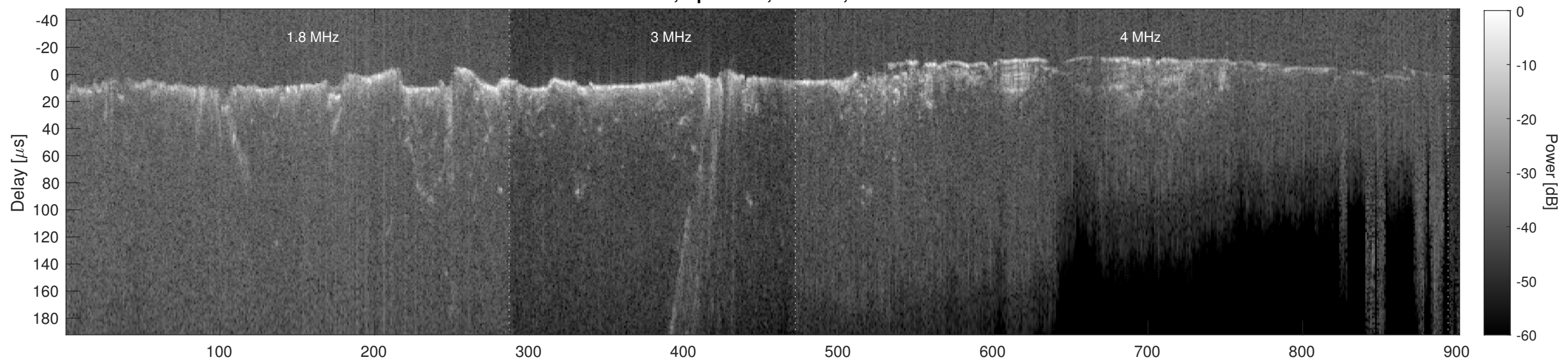
Orbit 6760, Cluttergram
