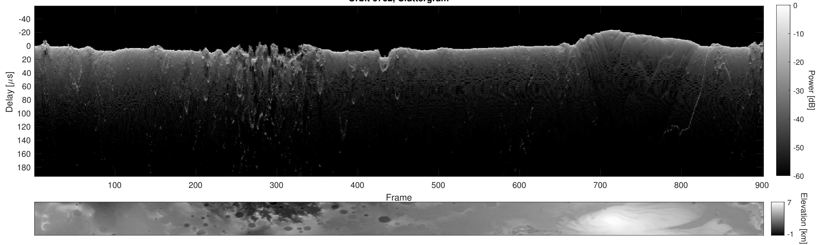
Orbit 6762, Cluttergram
