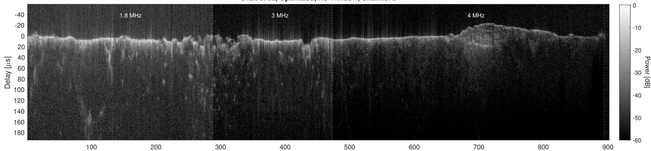
Orbit 6762, Cluttergram
