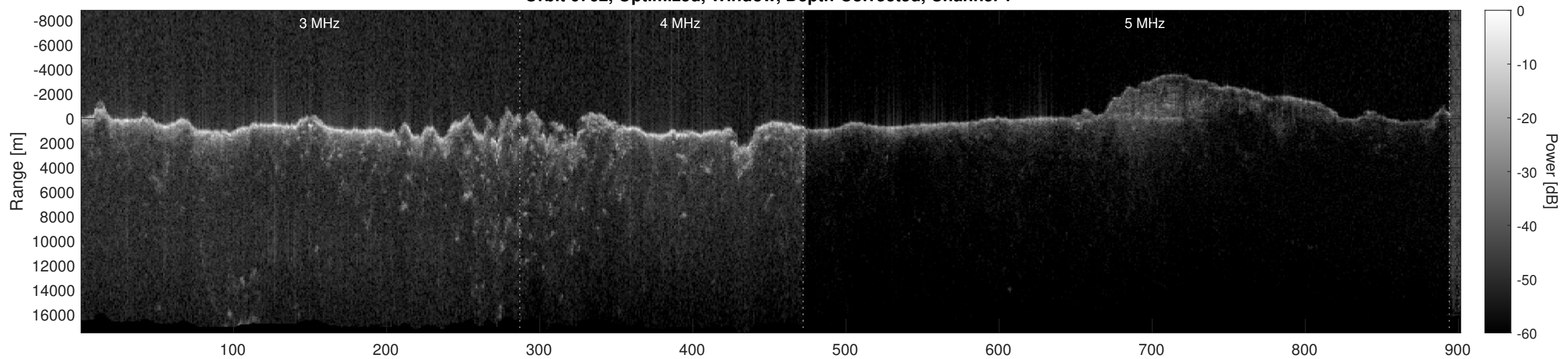
Orbit 6762, Optimized, Window, Depth-Corrected, Channel 2
