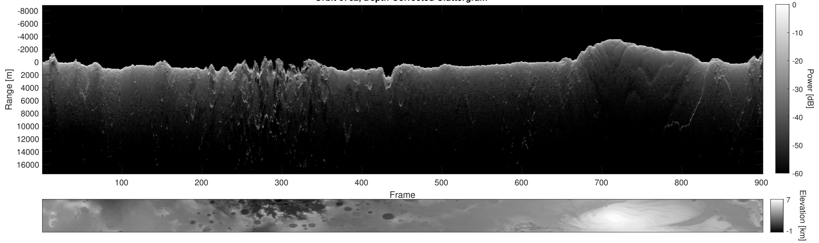
Orbit 6762, Depth-Corrected Cluttergram
