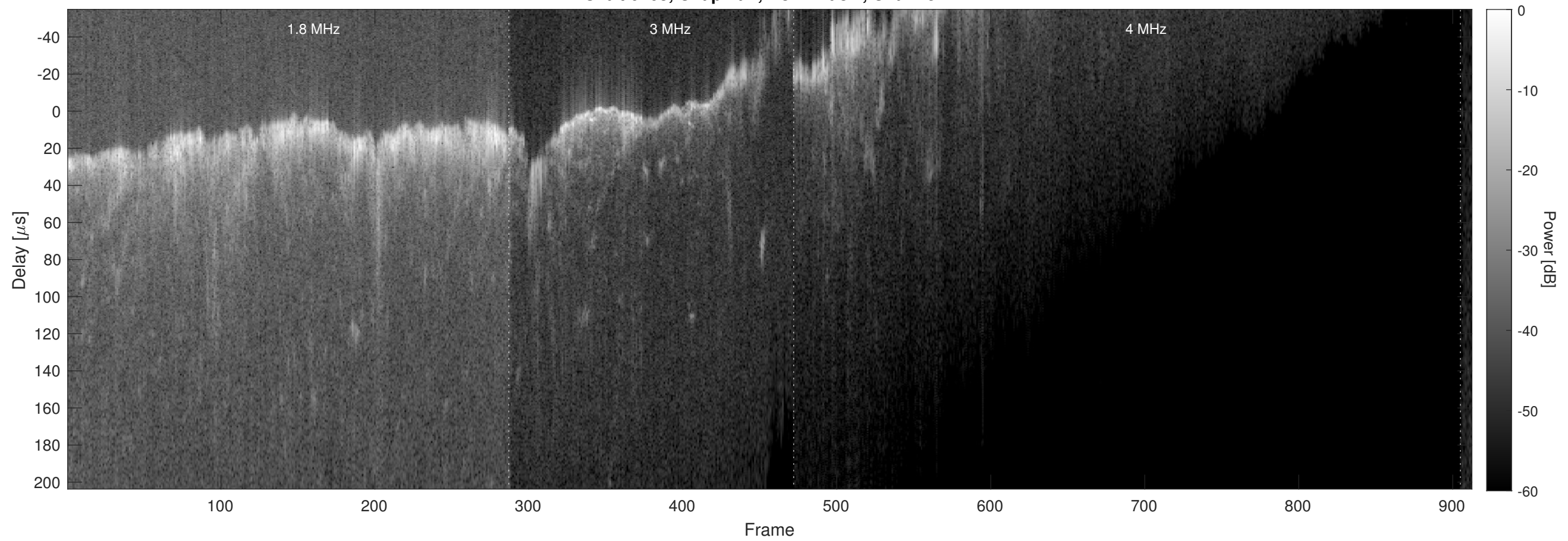
Orbit 6763, Chapman, No Window, Channel 2
