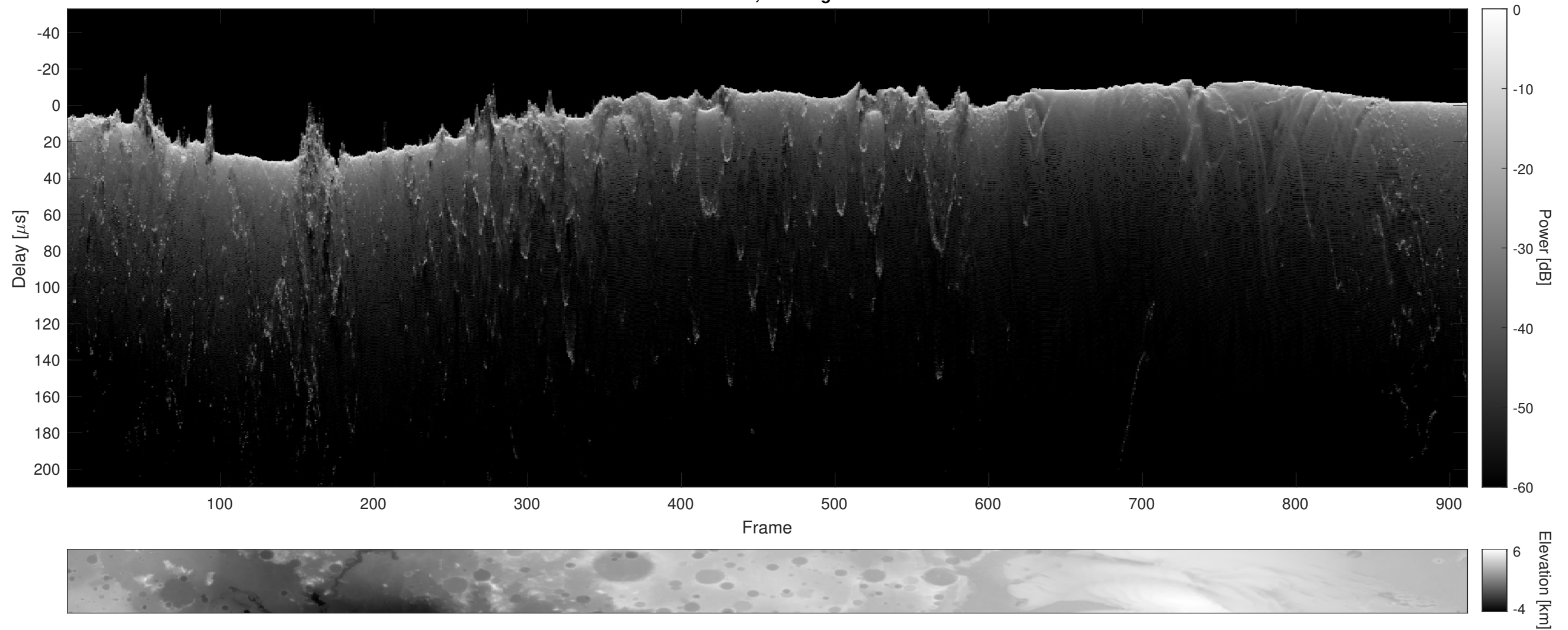
Orbit 6764, Cluttergram
