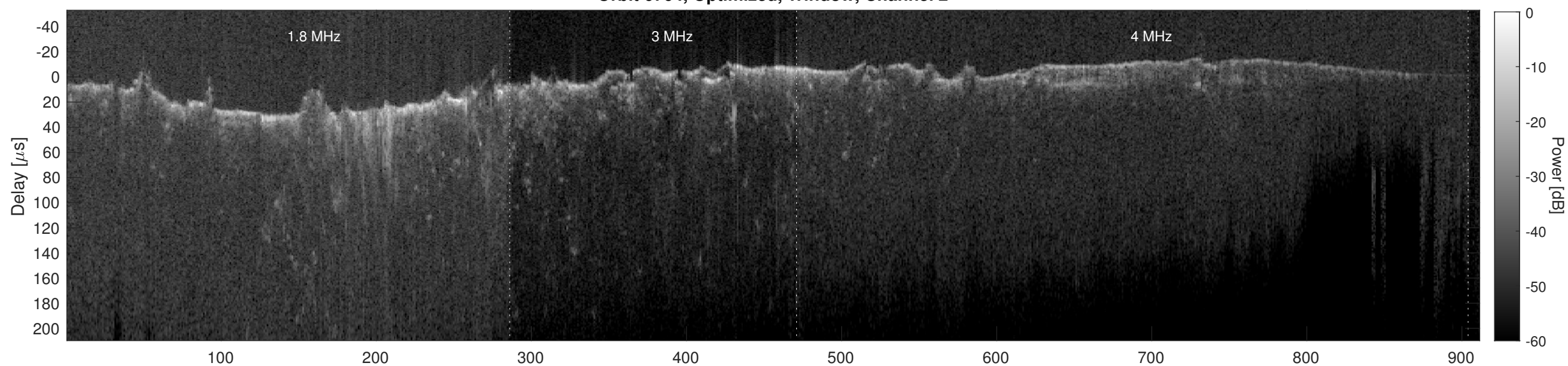
Orbit 6764, Cluttergram
