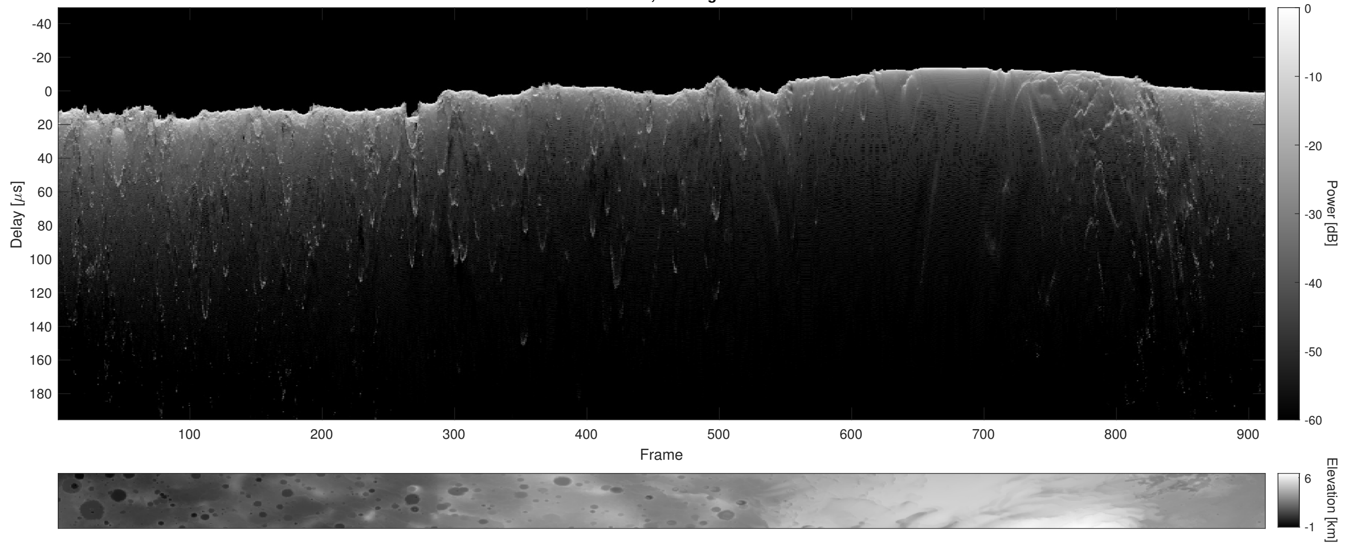
Orbit 6767, Cluttergram
