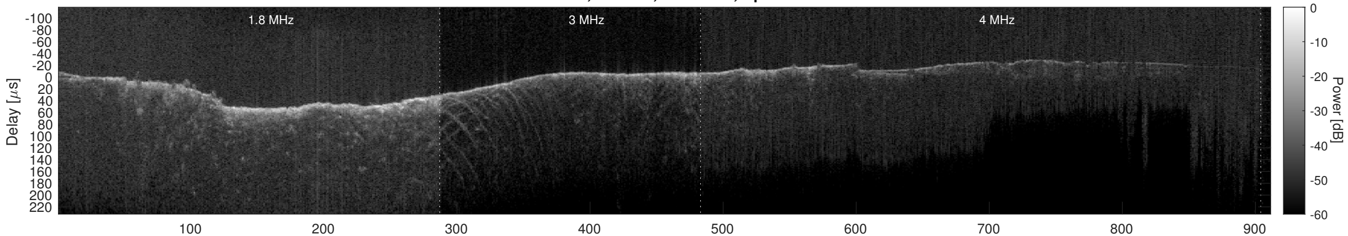
Orbit 6768, Cluttergram
