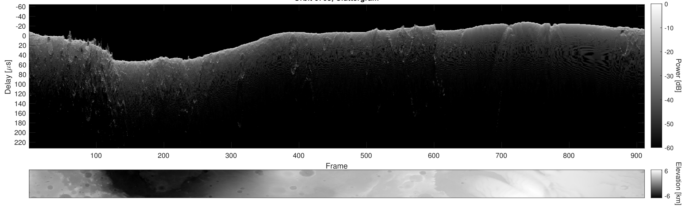
Orbit 6768, Cluttergram
