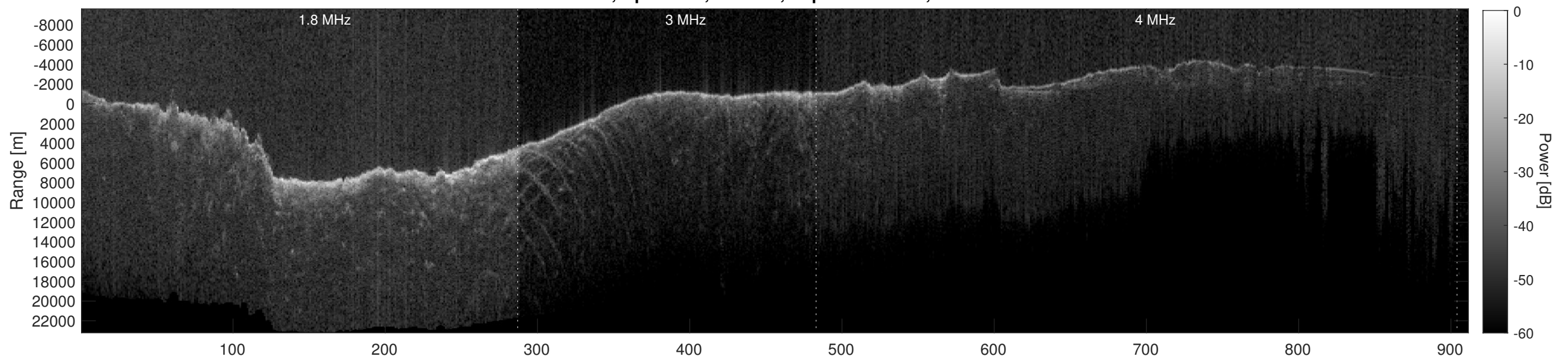
Orbit 6768, Depth-Corrected Cluttergram
