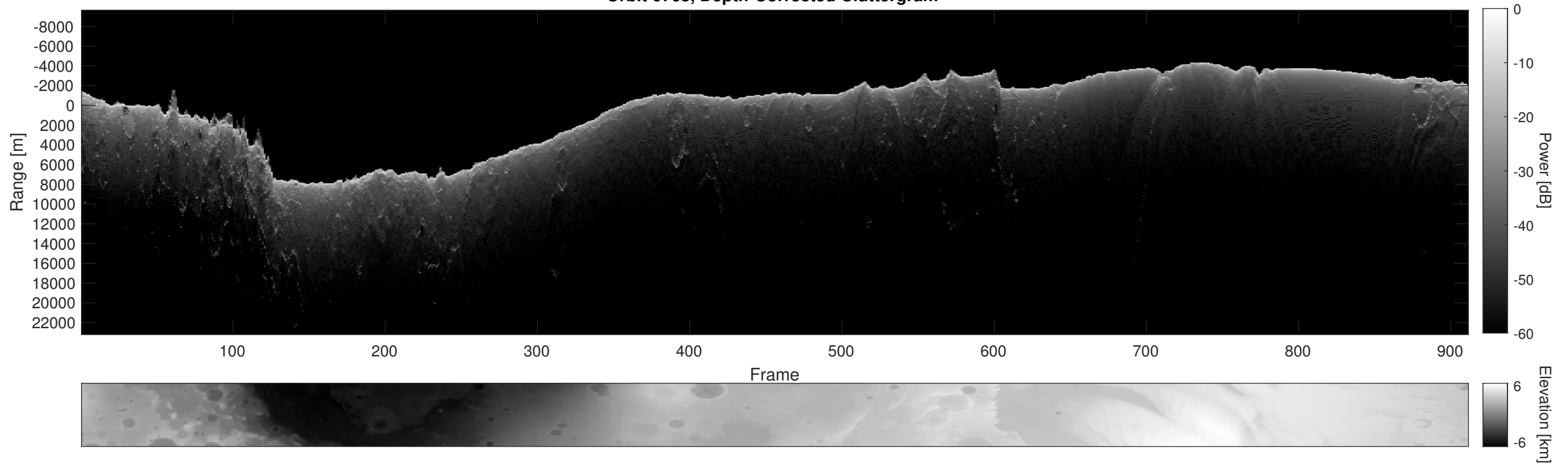
Orbit 6768, Depth-Corrected Cluttergram
