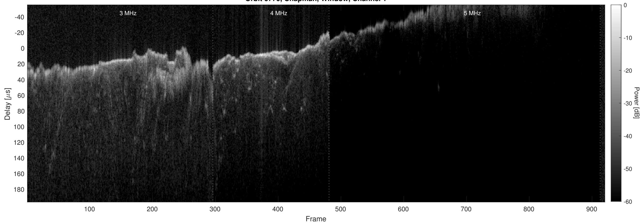
Orbit 6770, Chapman, Window, Channel 2
