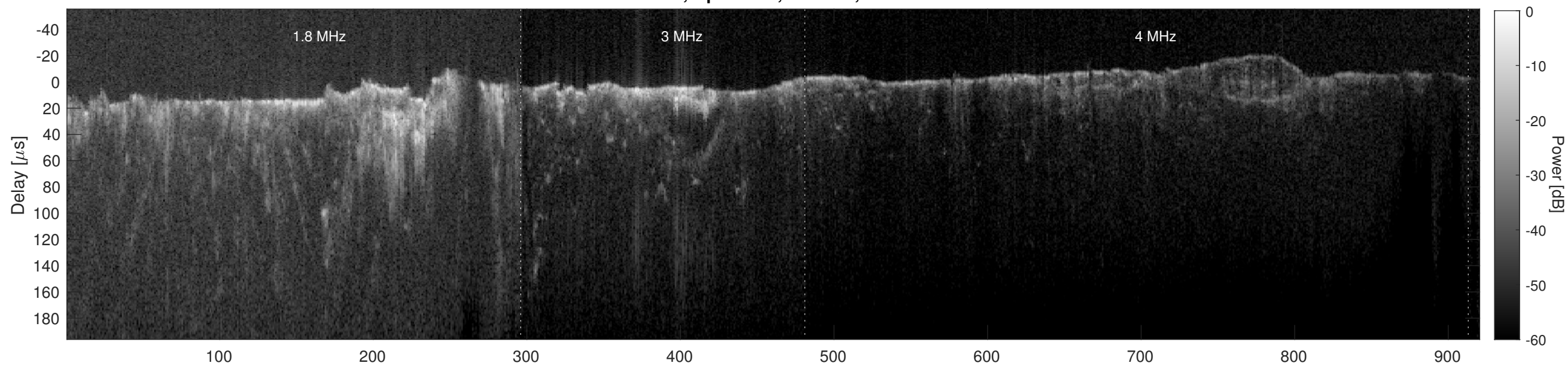
Orbit 6770, Cluttergram
