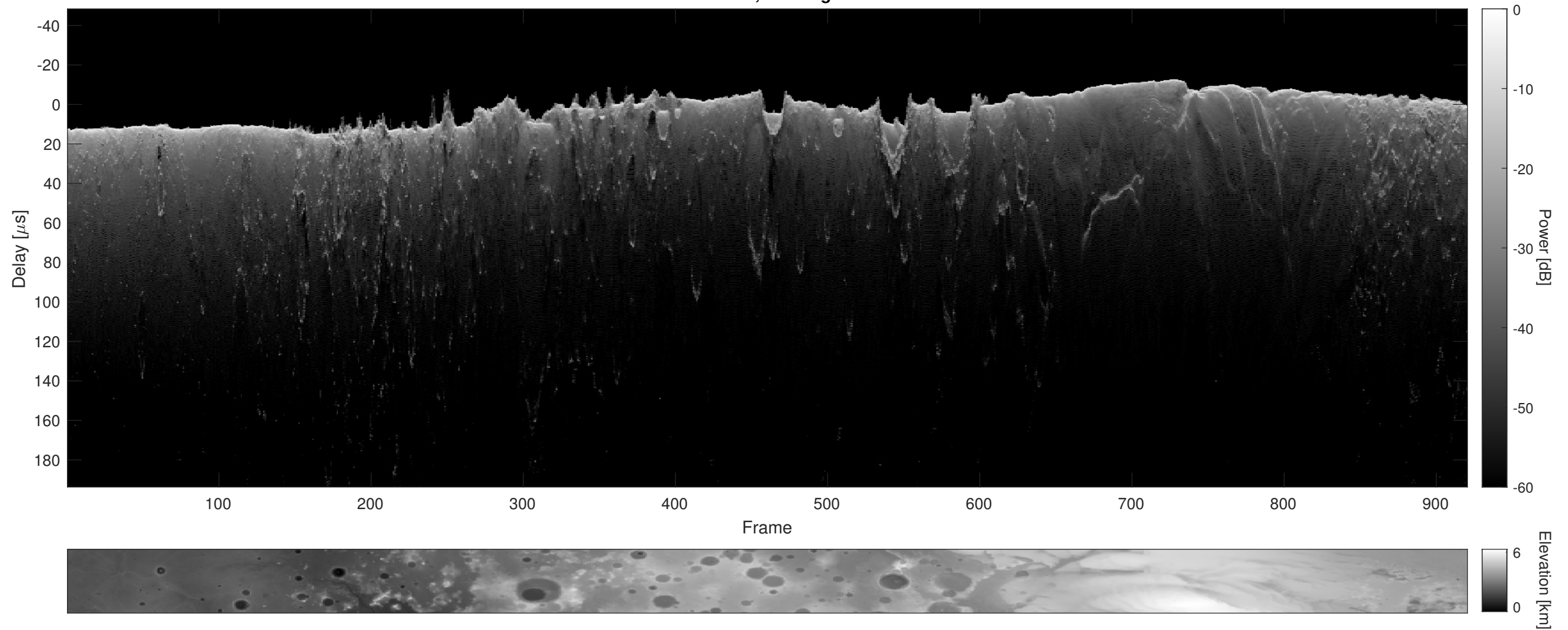
Orbit 6771, Cluttergram
