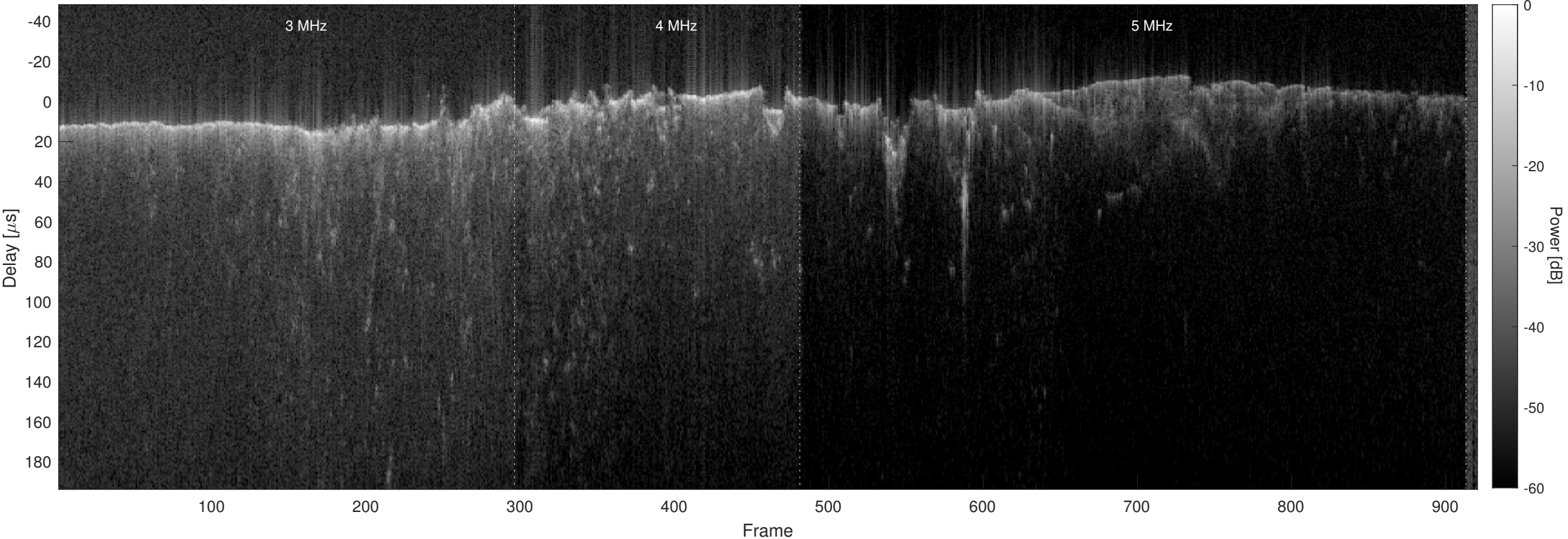
Orbit 6771, Optimized, No Window, Channel 2
