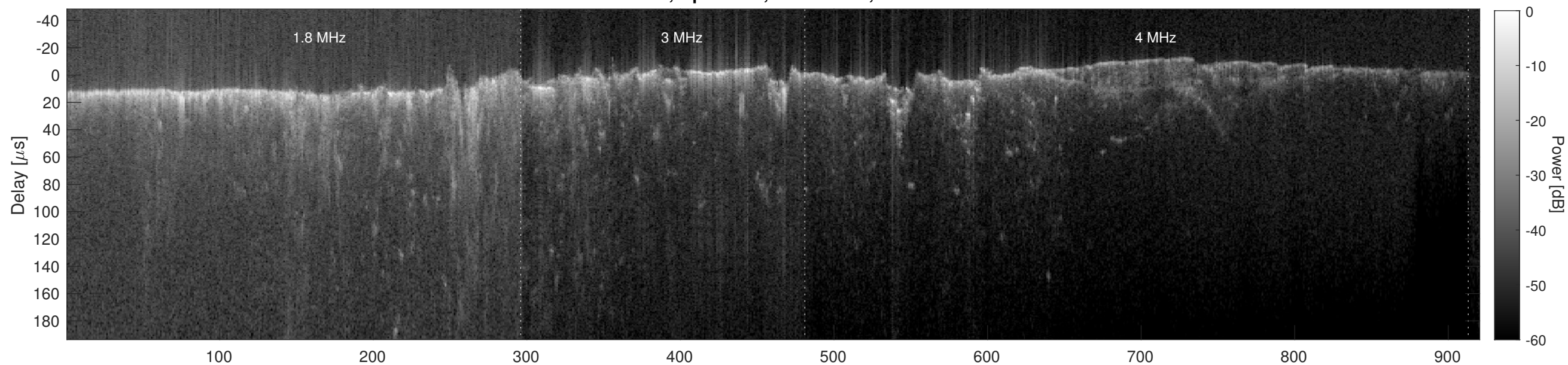
Orbit 6771, Cluttergram
