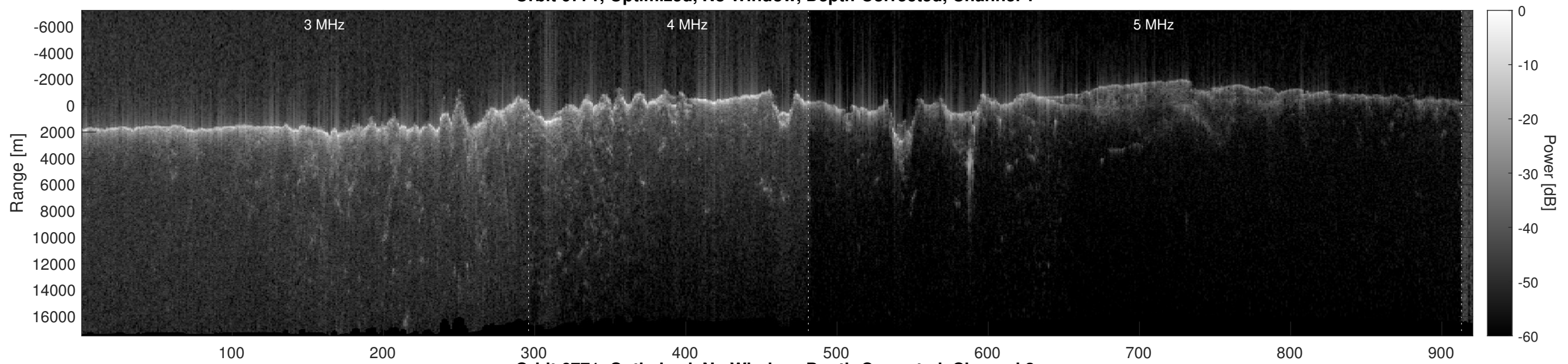
Orbit 6771, Optimized, No Window, Depth-Corrected, Channel 2
