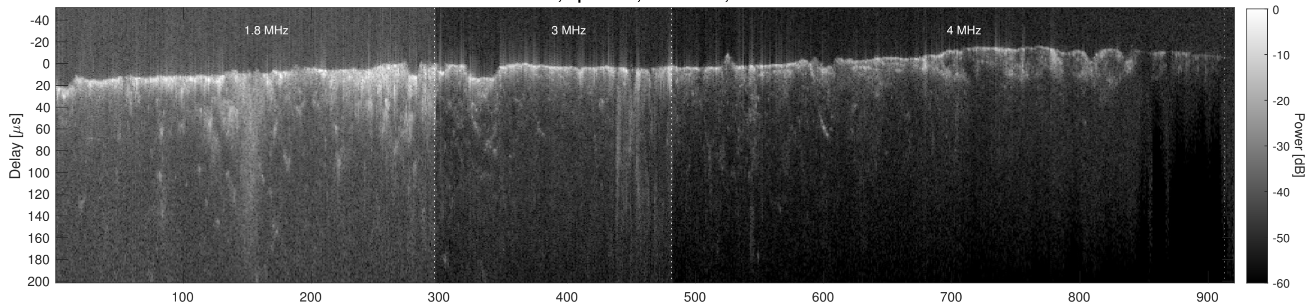
Orbit 6772, Cluttergram
