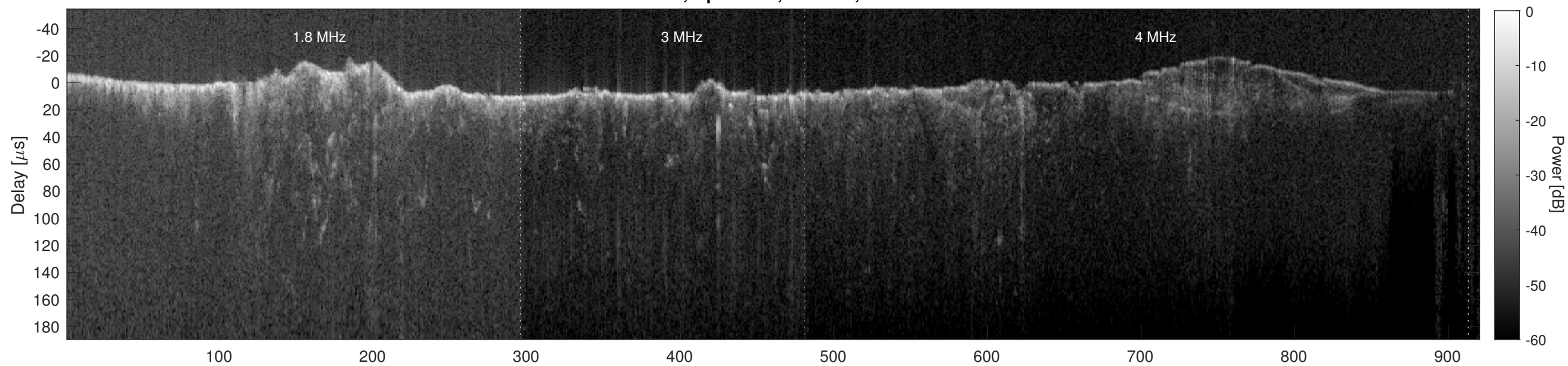
Orbit 6773, Cluttergram
