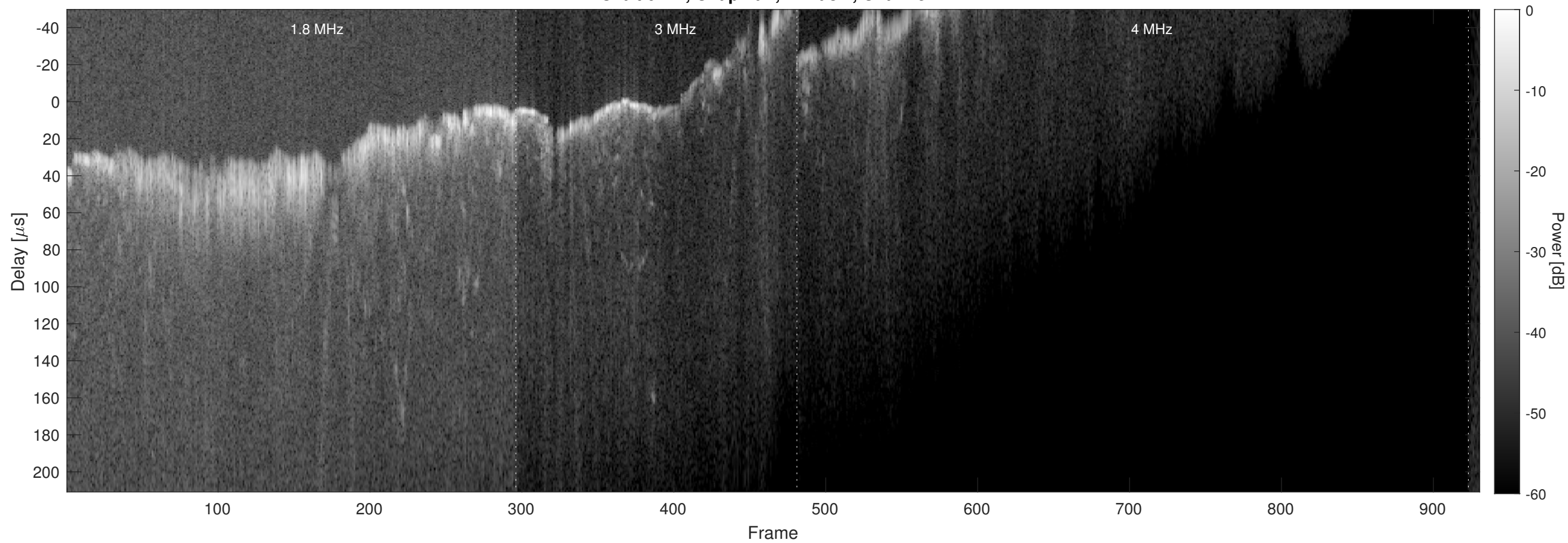
Orbit 6774, Chapman, Window, Channel 2
