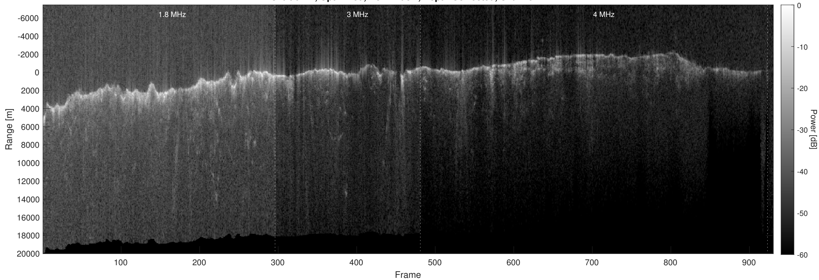
Orbit 6774, Optimized, No Window, Depth-Corrected, Channel 2
