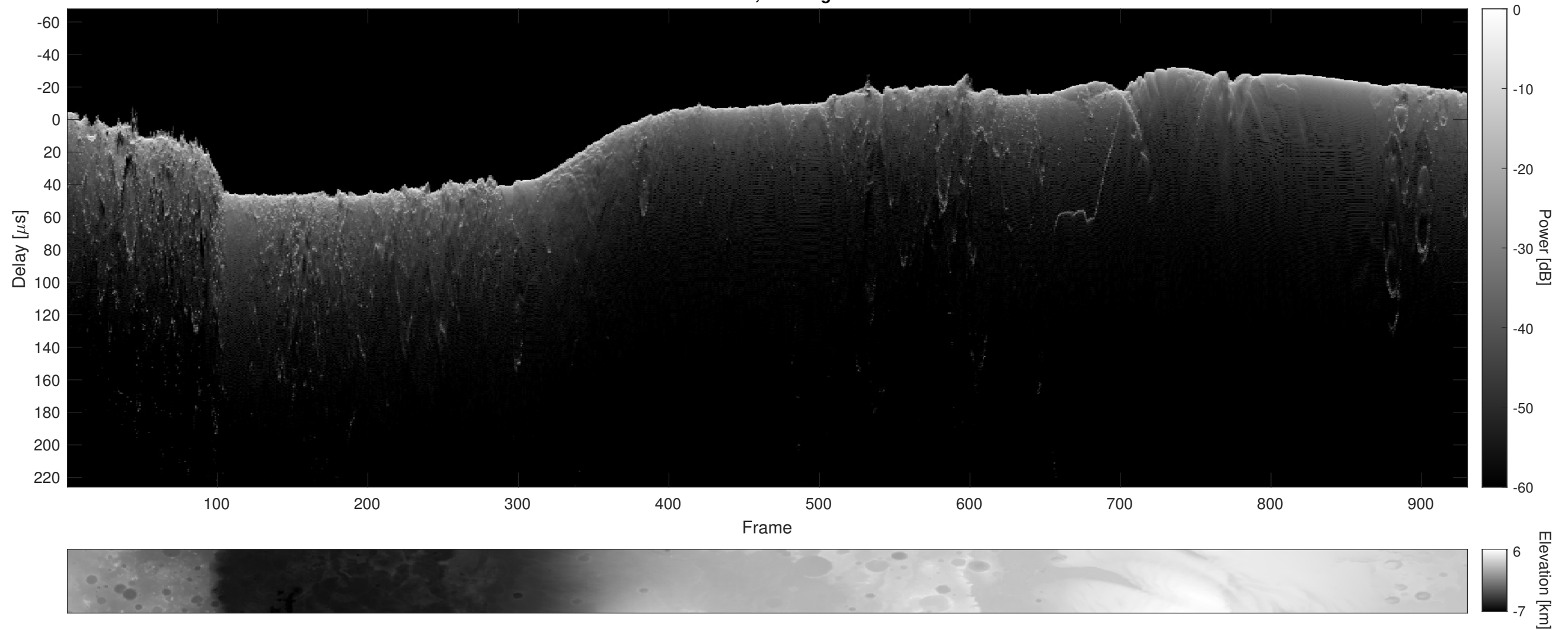
Orbit 6775, Cluttergram
