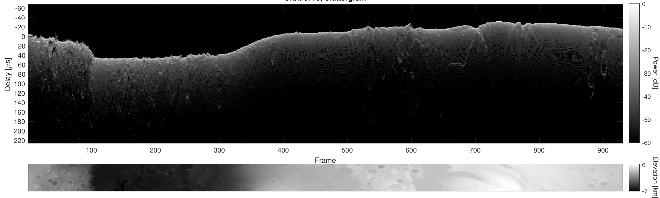
Orbit 6775, Cluttergram
