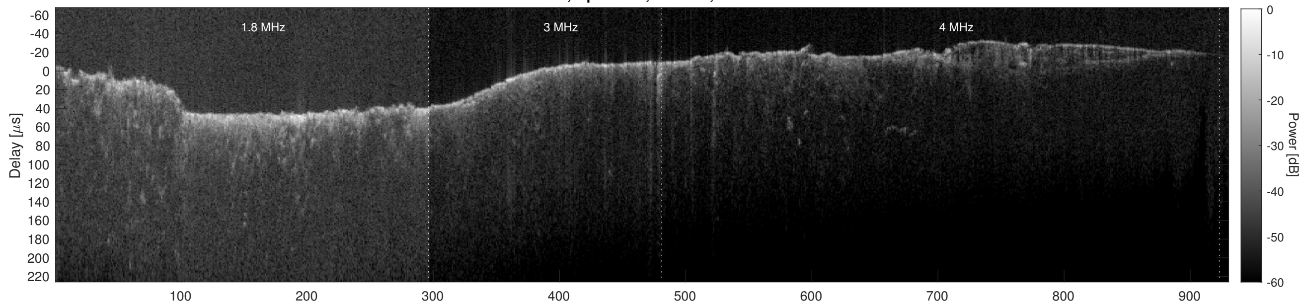
Orbit 6775, Cluttergram
