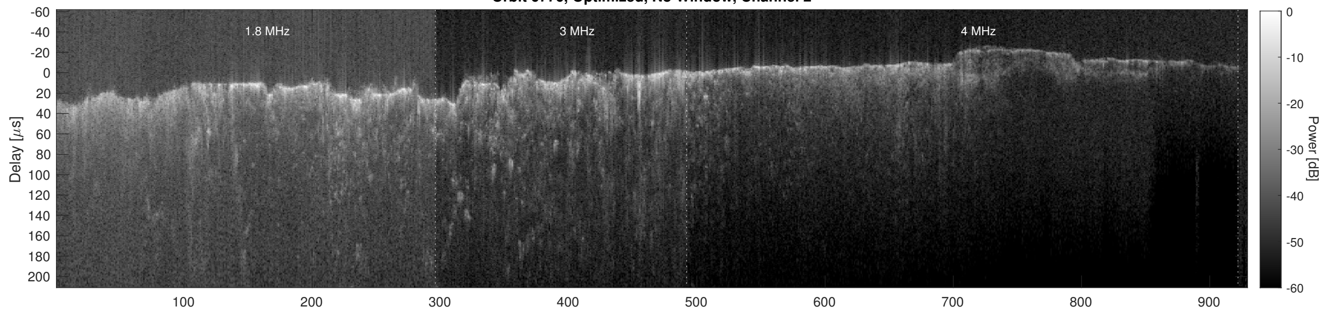
Orbit 6776, Cluttergram
