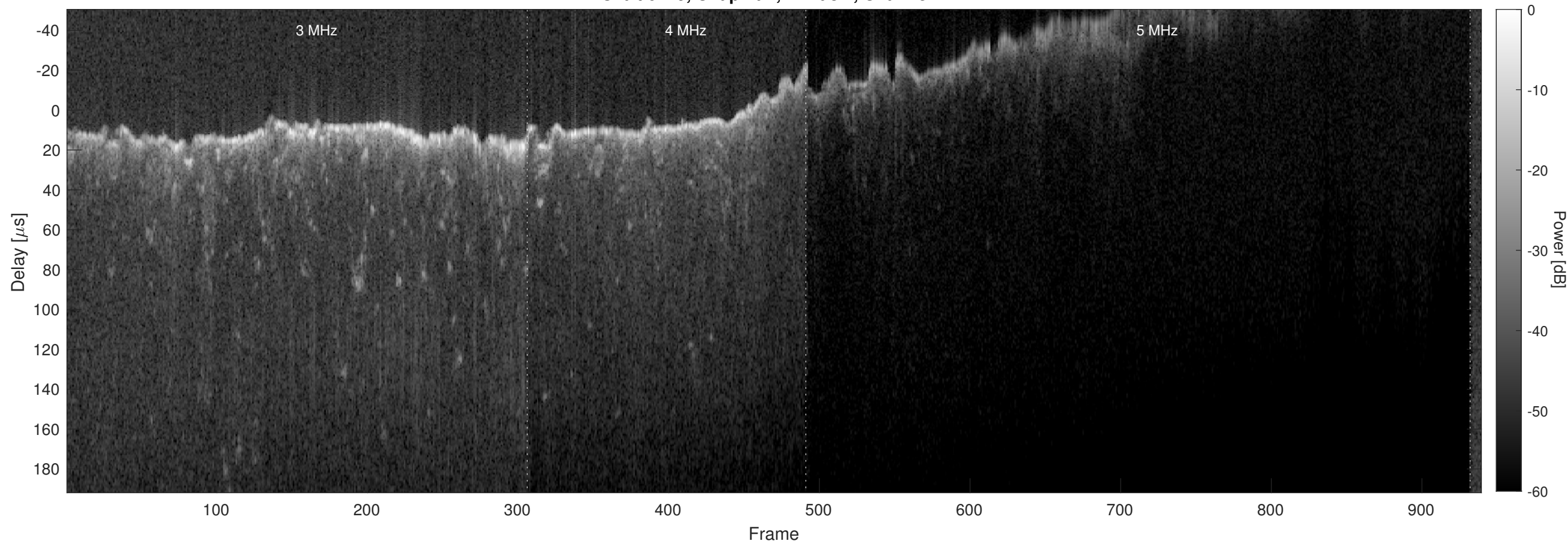
Orbit 6779, Chapman, Window, Channel 2
