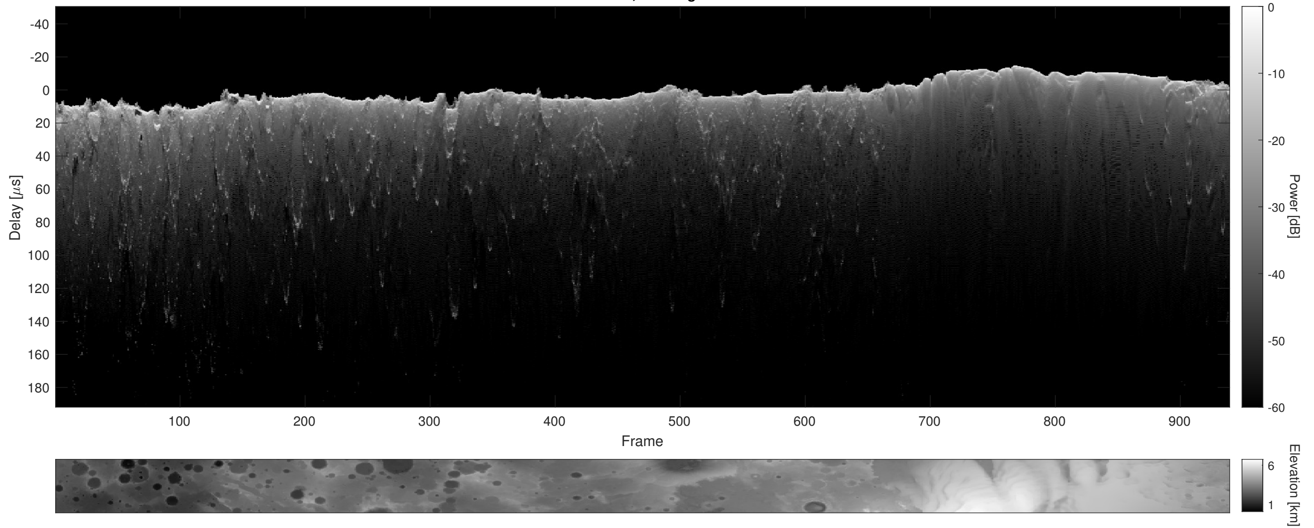
Orbit 6779, Cluttergram
