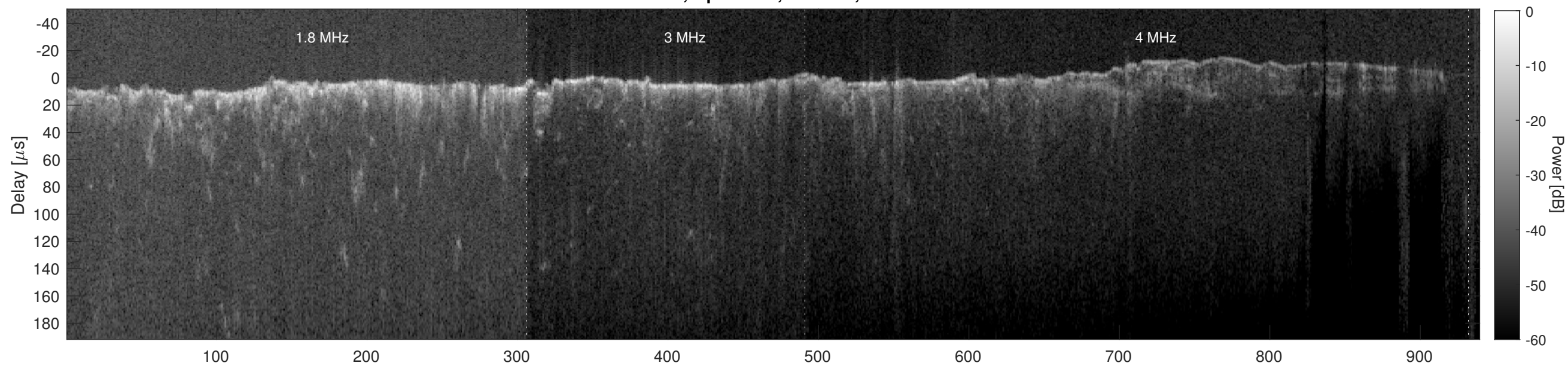
Orbit 6779, Cluttergram
