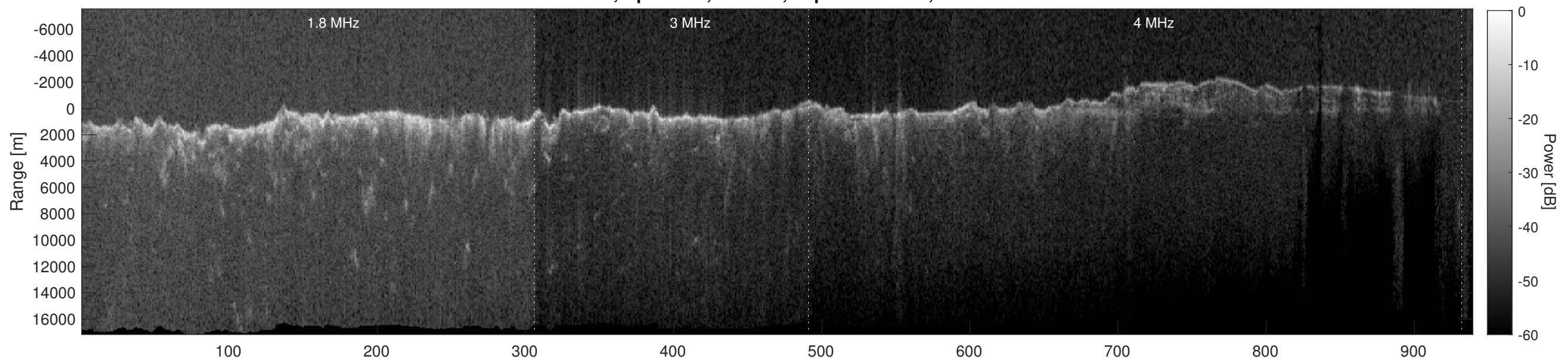
Orbit 6779, Depth-Corrected Cluttergram
