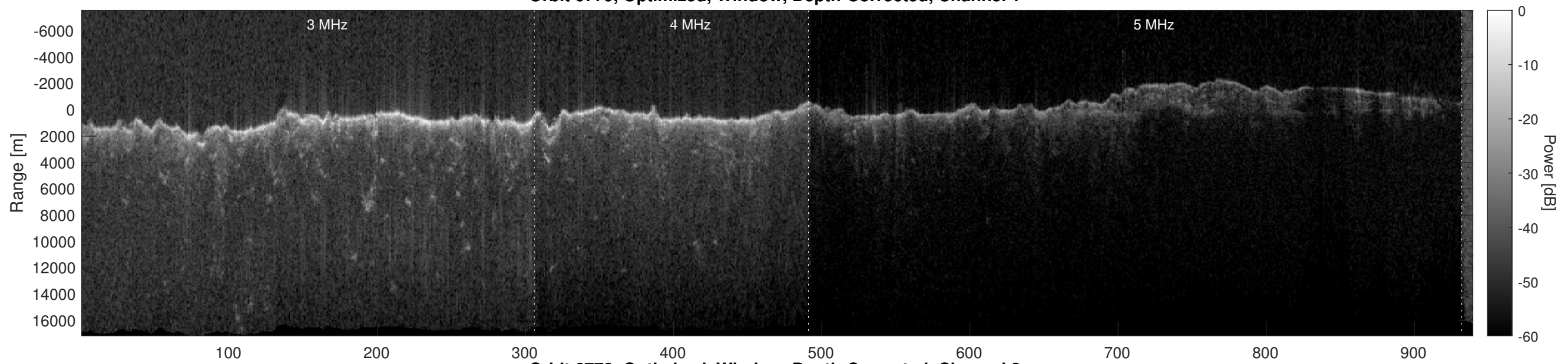
Orbit 6779, Optimized, Window, Depth-Corrected, Channel 2
