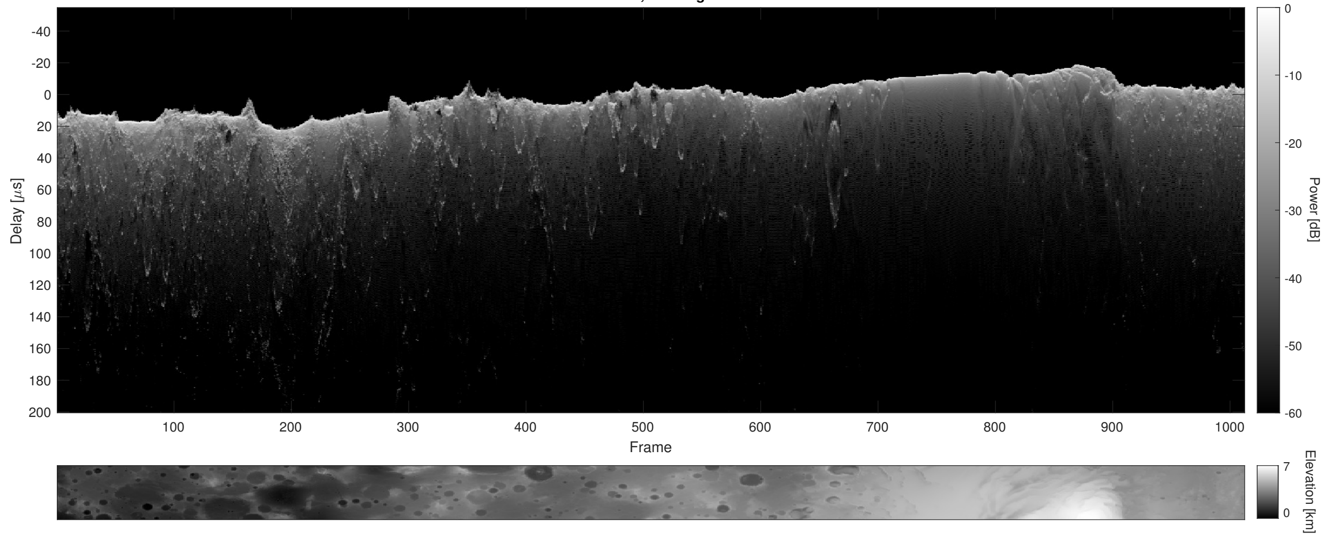
Orbit 6781, Cluttergram
