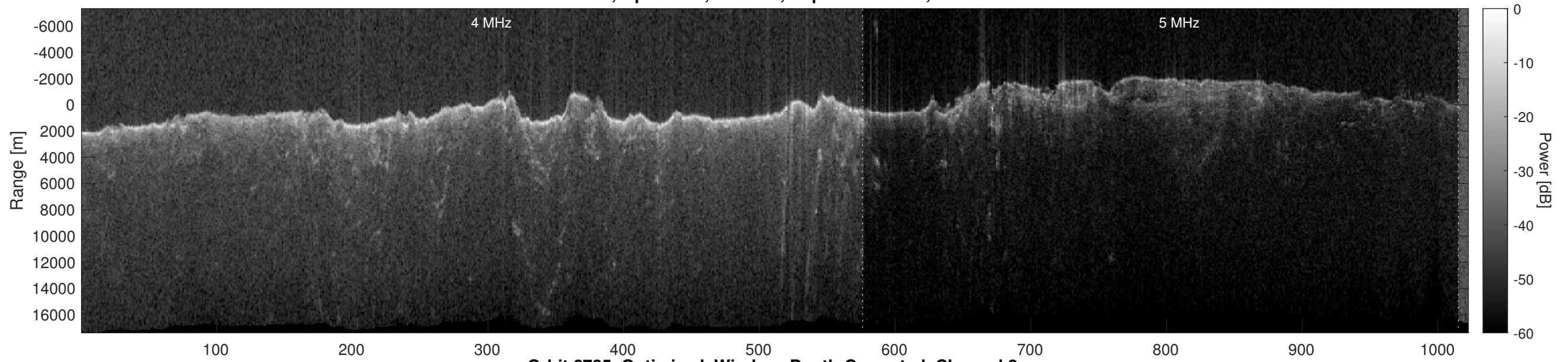
Orbit 6785, Optimized, Window, Depth-Corrected, Channel 2
