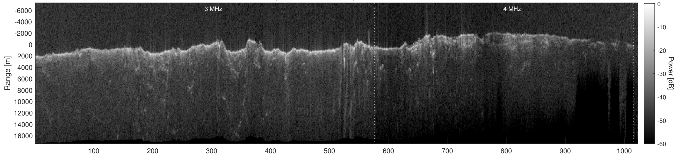
Orbit 6785, Depth-Corrected Cluttergram
