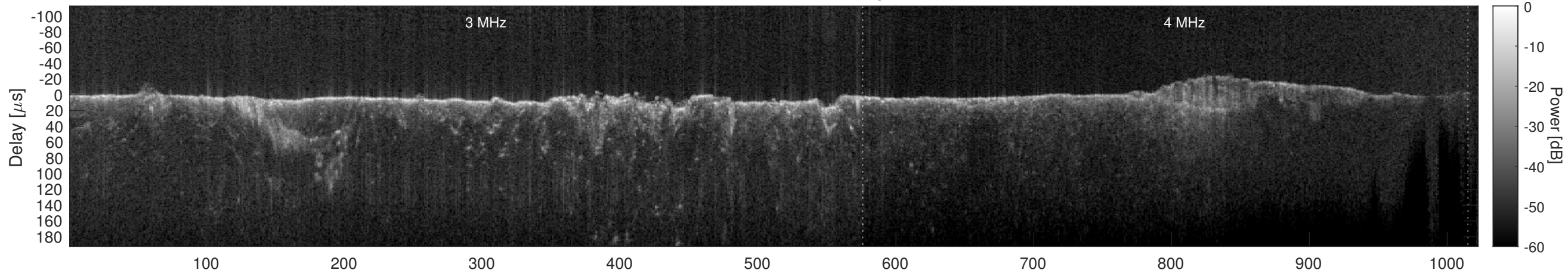
Orbit 6787, Cluttergram
