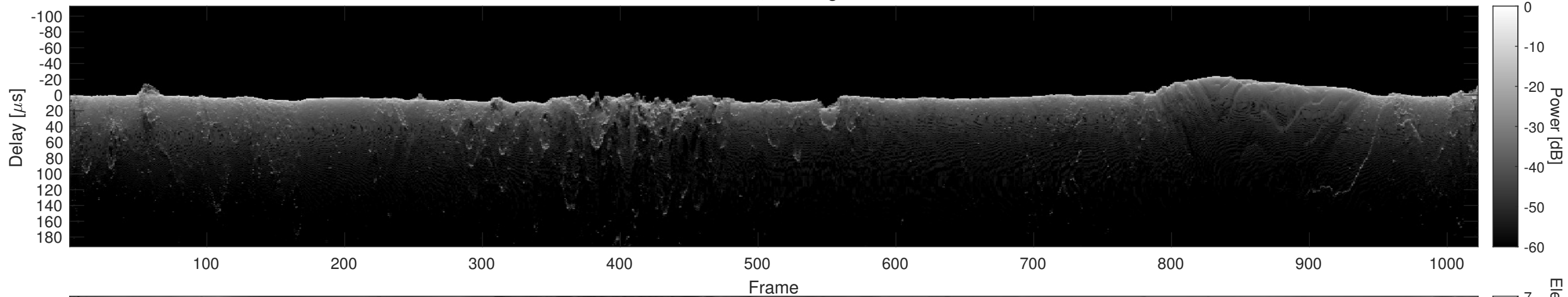
Orbit 6787, Cluttergram
