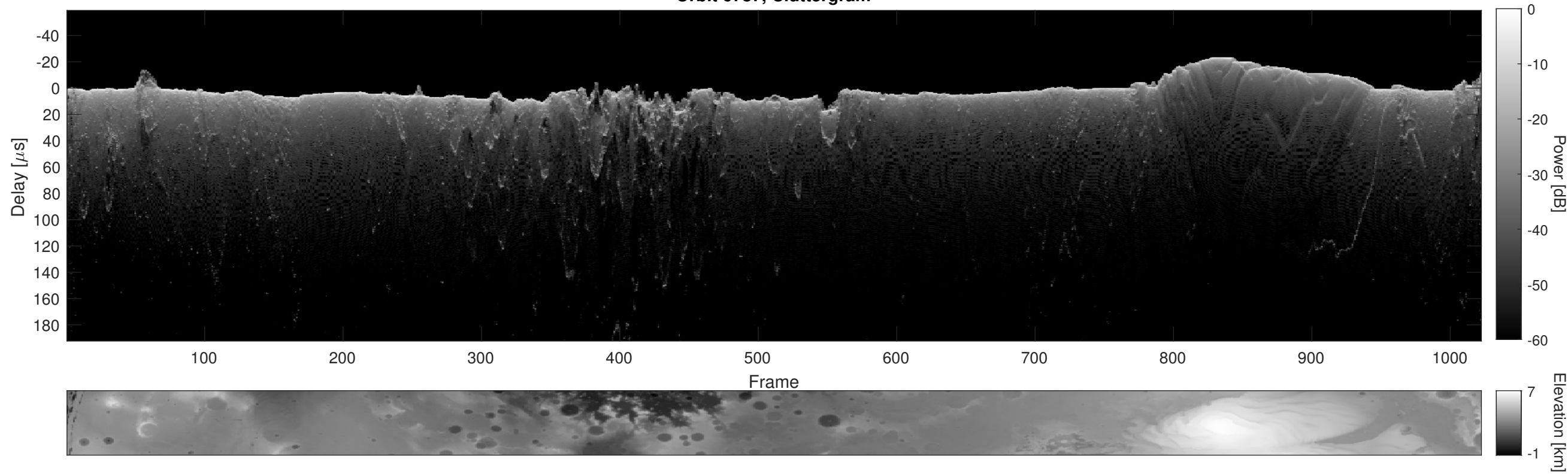
Orbit 6787, Cluttergram
