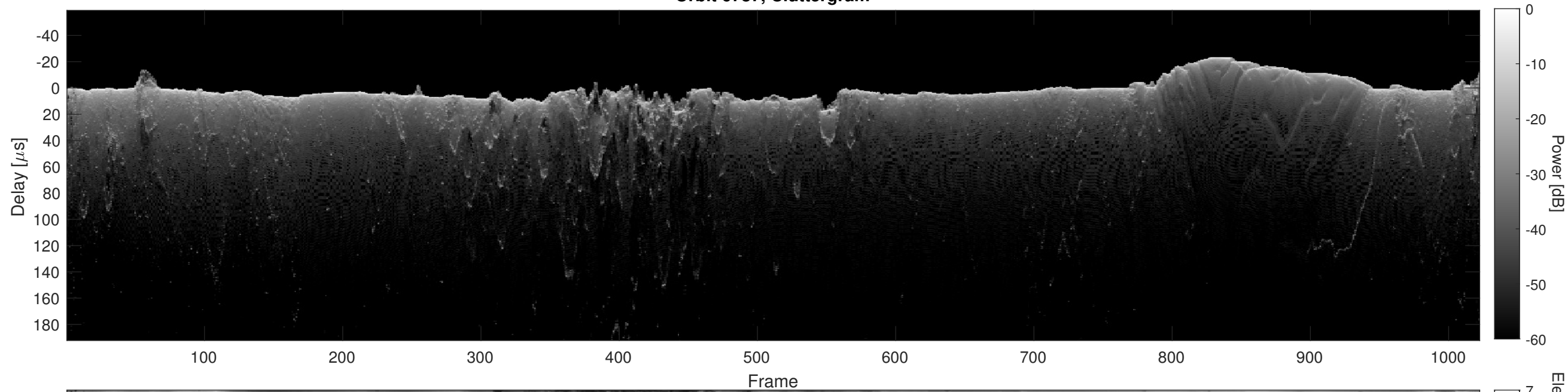
Orbit 6787, Cluttergram
