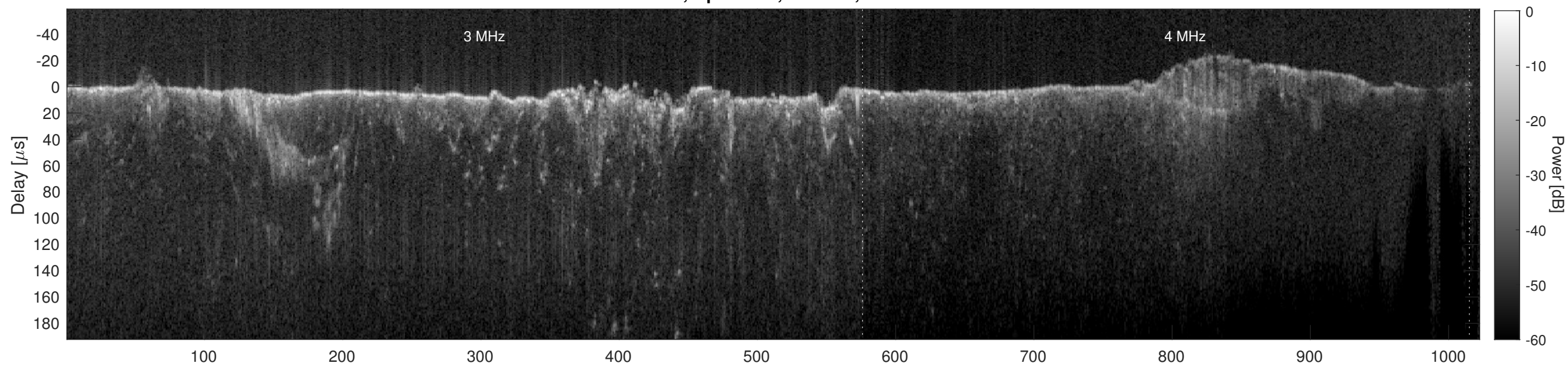
Orbit 6787, Cluttergram
