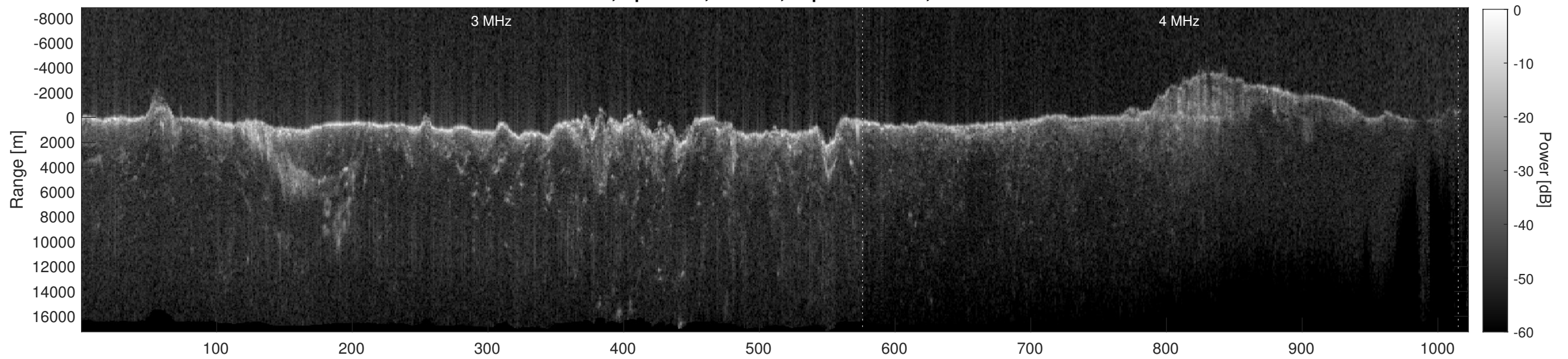
Orbit 6787, Depth-Corrected Cluttergram
