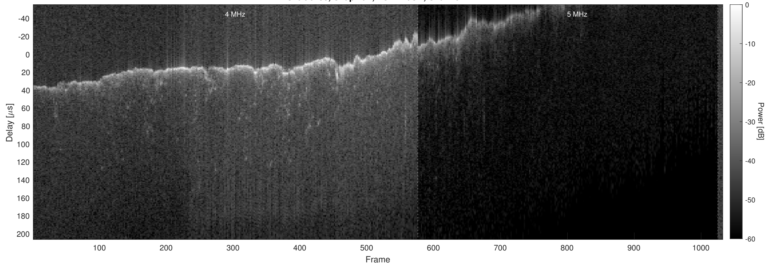
Orbit 6790, Chapman, No Window, Channel 2
