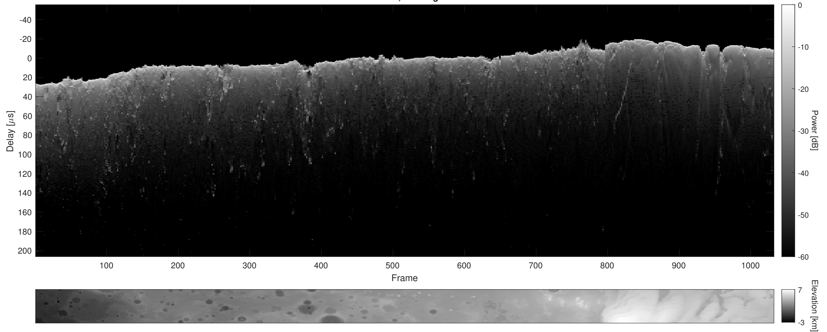
Orbit 6790, Cluttergram
