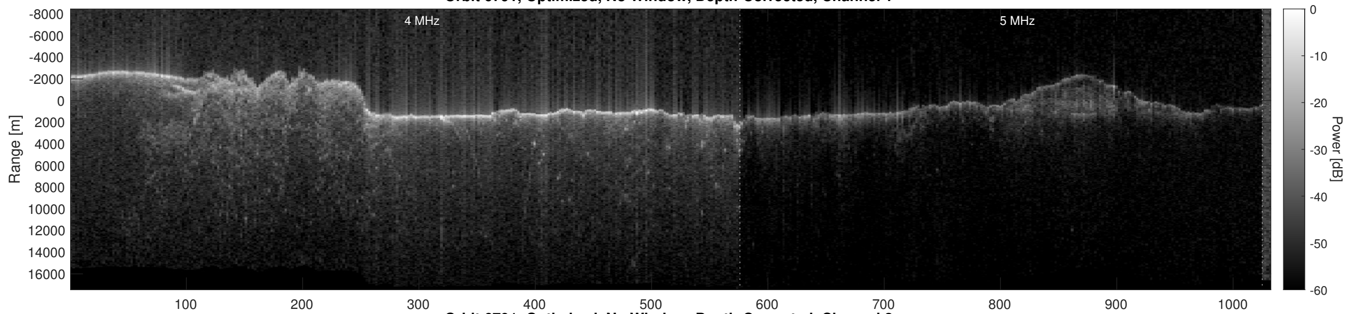
Orbit 6791, Optimized, No Window, Depth-Corrected, Channel 2
