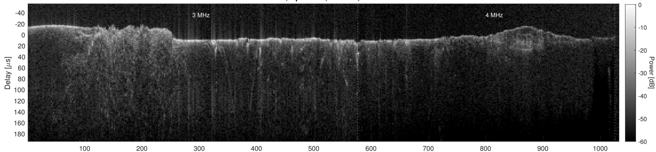
Orbit 6791, Cluttergram
